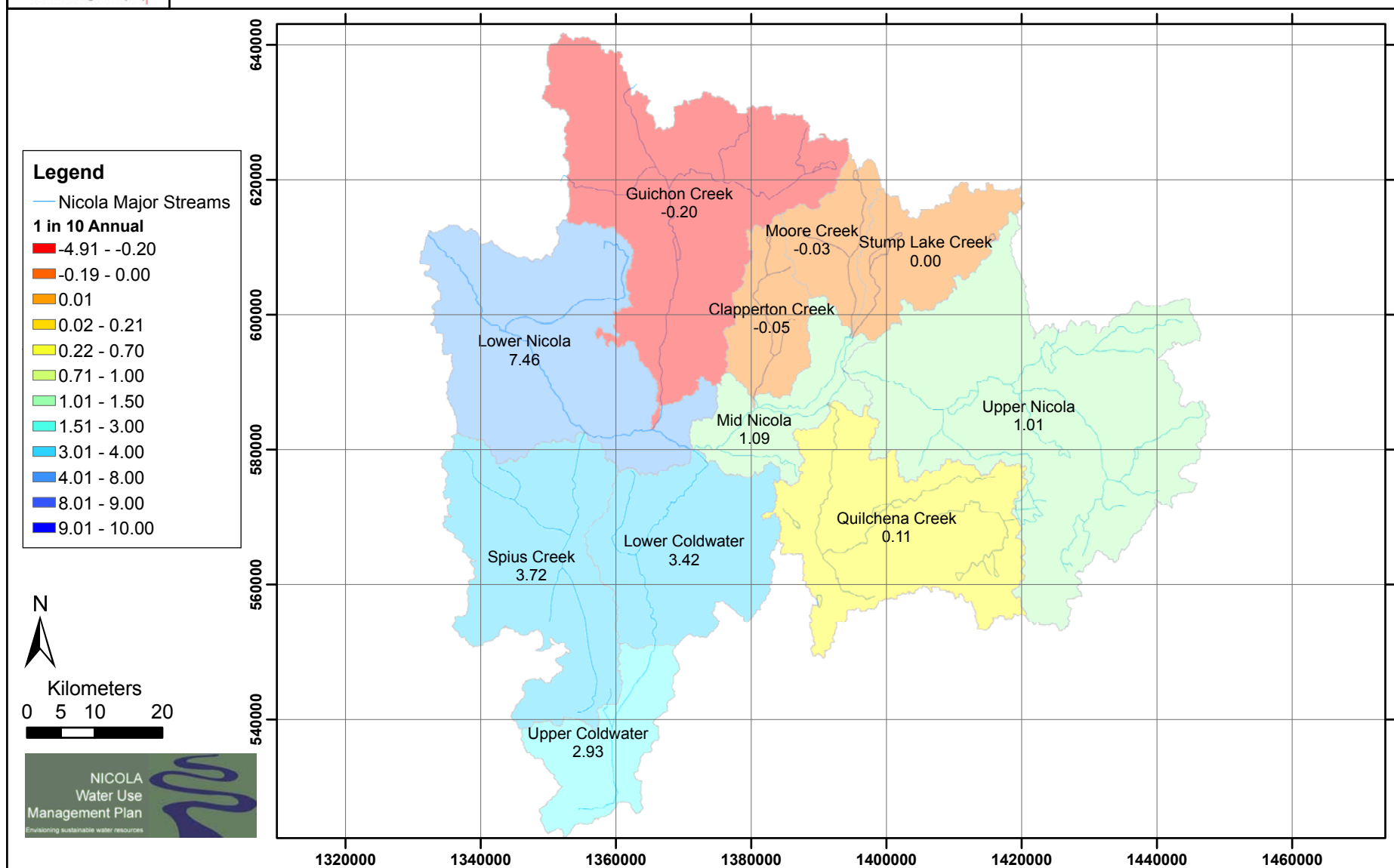
Figure 8 2050 Conditions: Annual water budget in m 3 /s for 1 in 10 year drought
