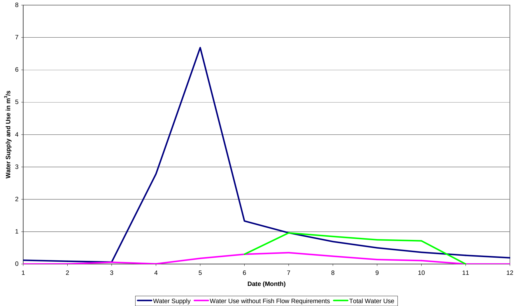
Figure 15: Water Supply and Use for Typical 1 in 10 year Drought Conditions Quilchena
