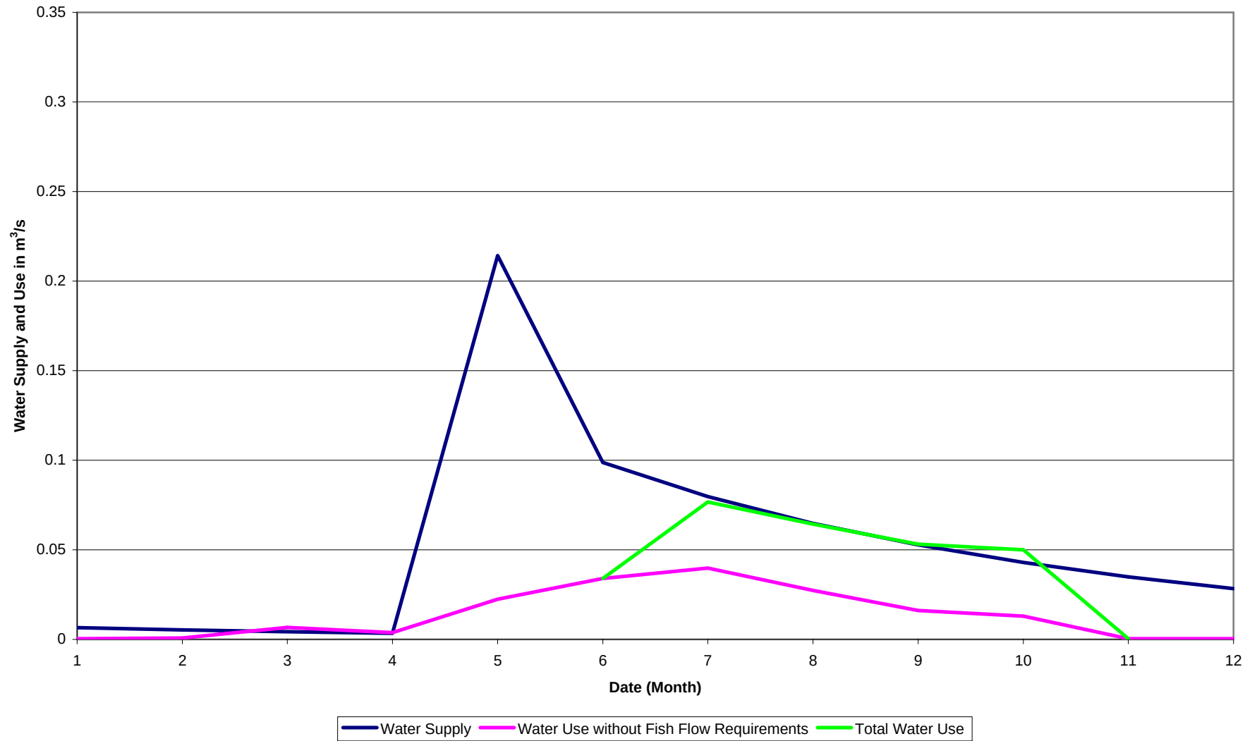
Figure 14: Water Supply and Use for Typical 1 in 10 year Drought Conditions Moore
