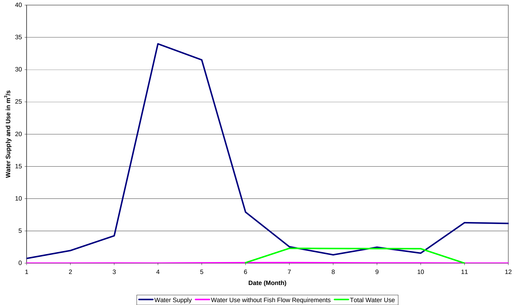
Figure 16: Water Supply and Use for Typical 1 in 10 year Drought Conditions Spius
