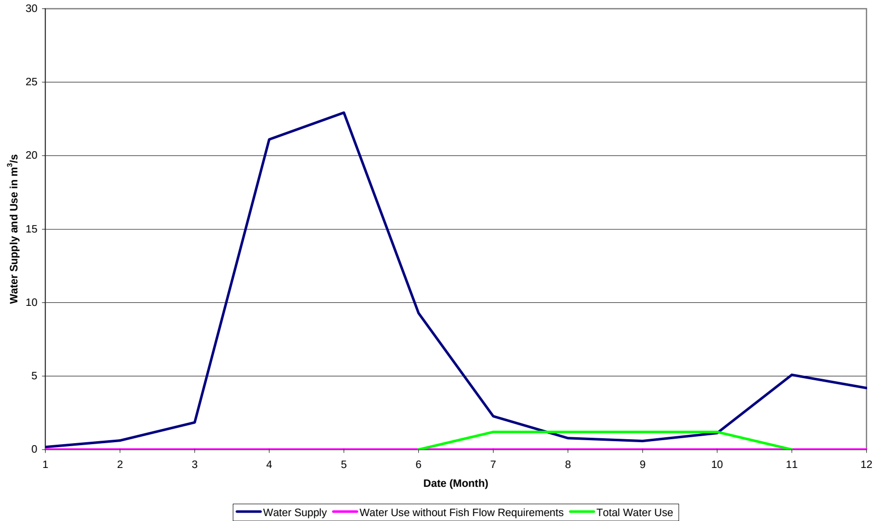
Figure 18: Water Supply and Use for Typical 1 in 10 year Drought Conditions Upper Coldwater
