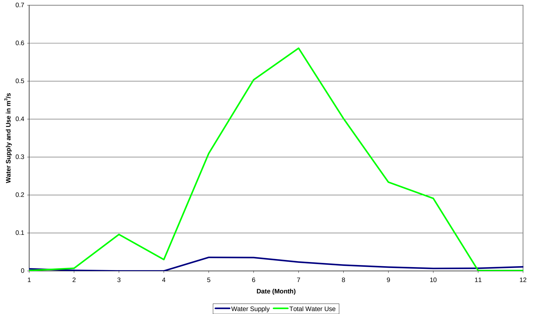
Figure 17: Water Supply and Use for Typical 1 in 10 year Drought Conditions Stump
