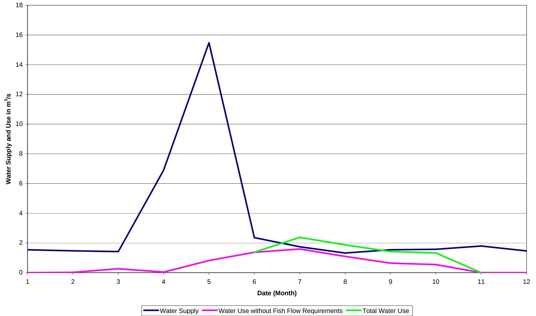
Figure 19: Water Supply and Use for Typical 1 in 10 year Drought Conditions Upper Nicola
