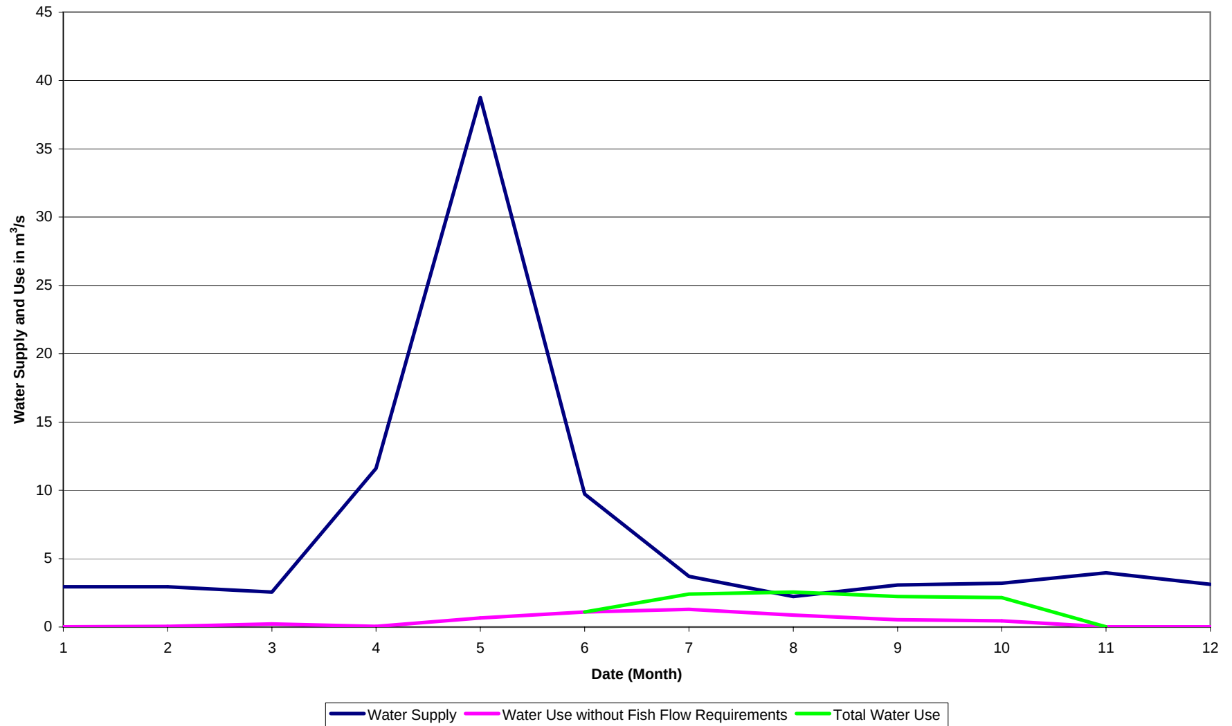
Figure 13: Water Supply and Use for Typical 1 in 10 year Drought Conditions Middle Nicola
