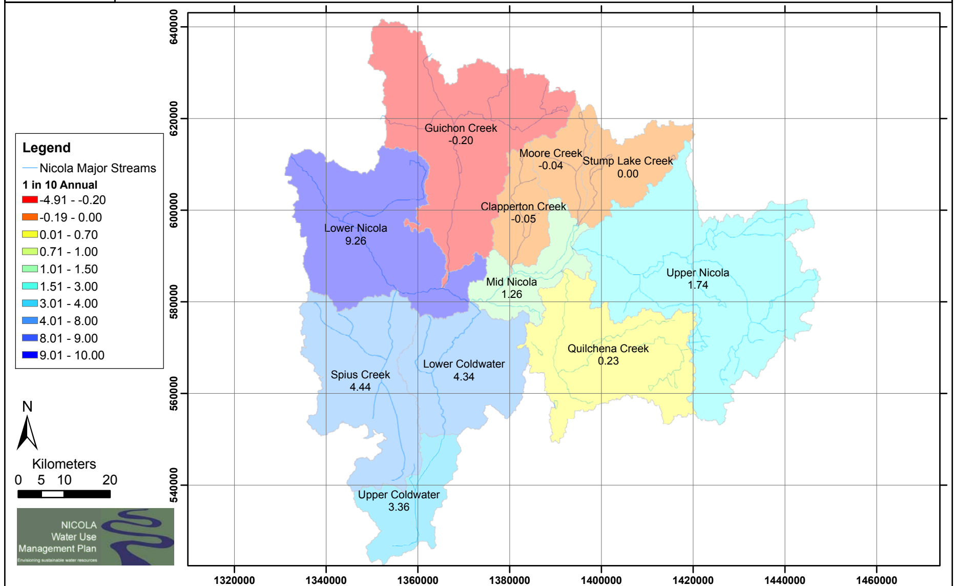
Figure 6 2020 Conditions: Annual water budget in m 3 /s for 1 in 10 year drought
