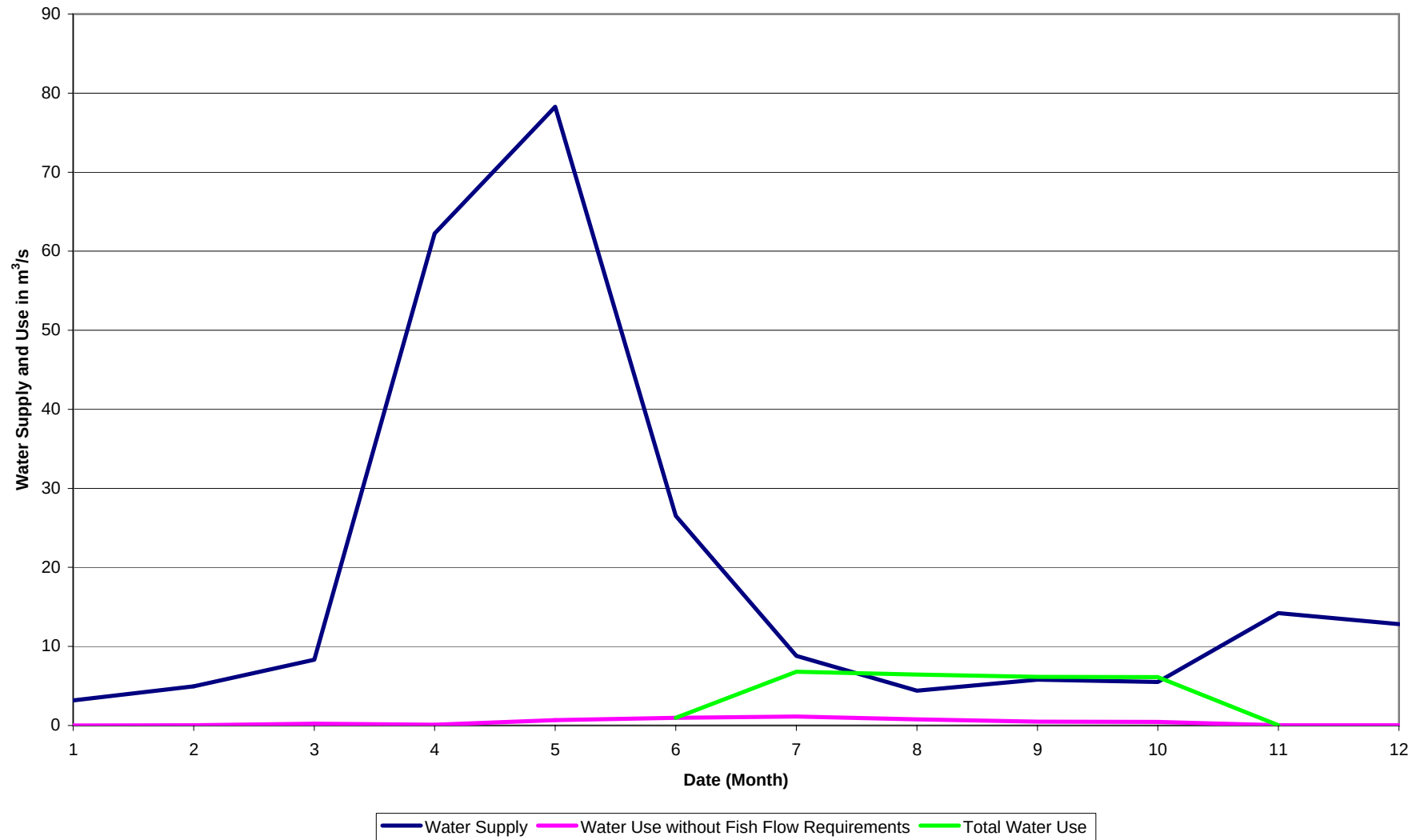
Figure 12: Water Supply and Use for Typical 1 in 10 year Drought Conditions Lower Nicola
