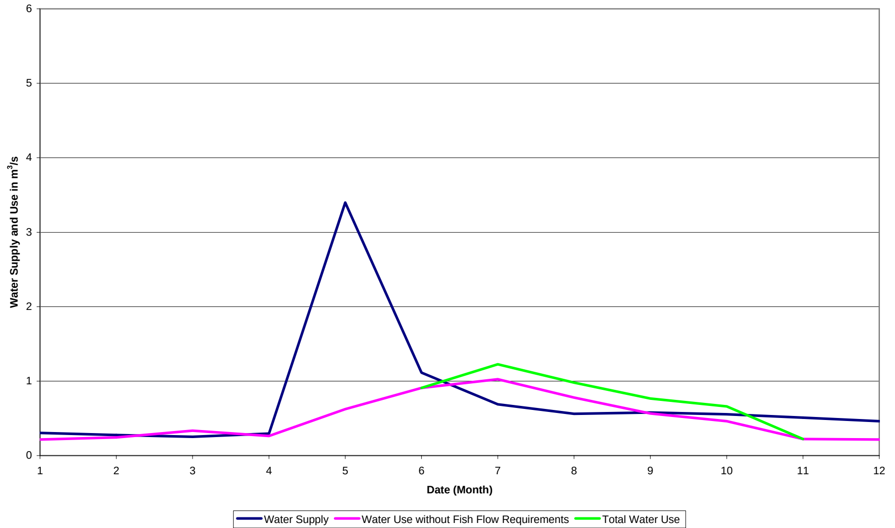
Figure 10: Water Supply and Use for Typical 1 in 10 year Drought Conditions Guichon
