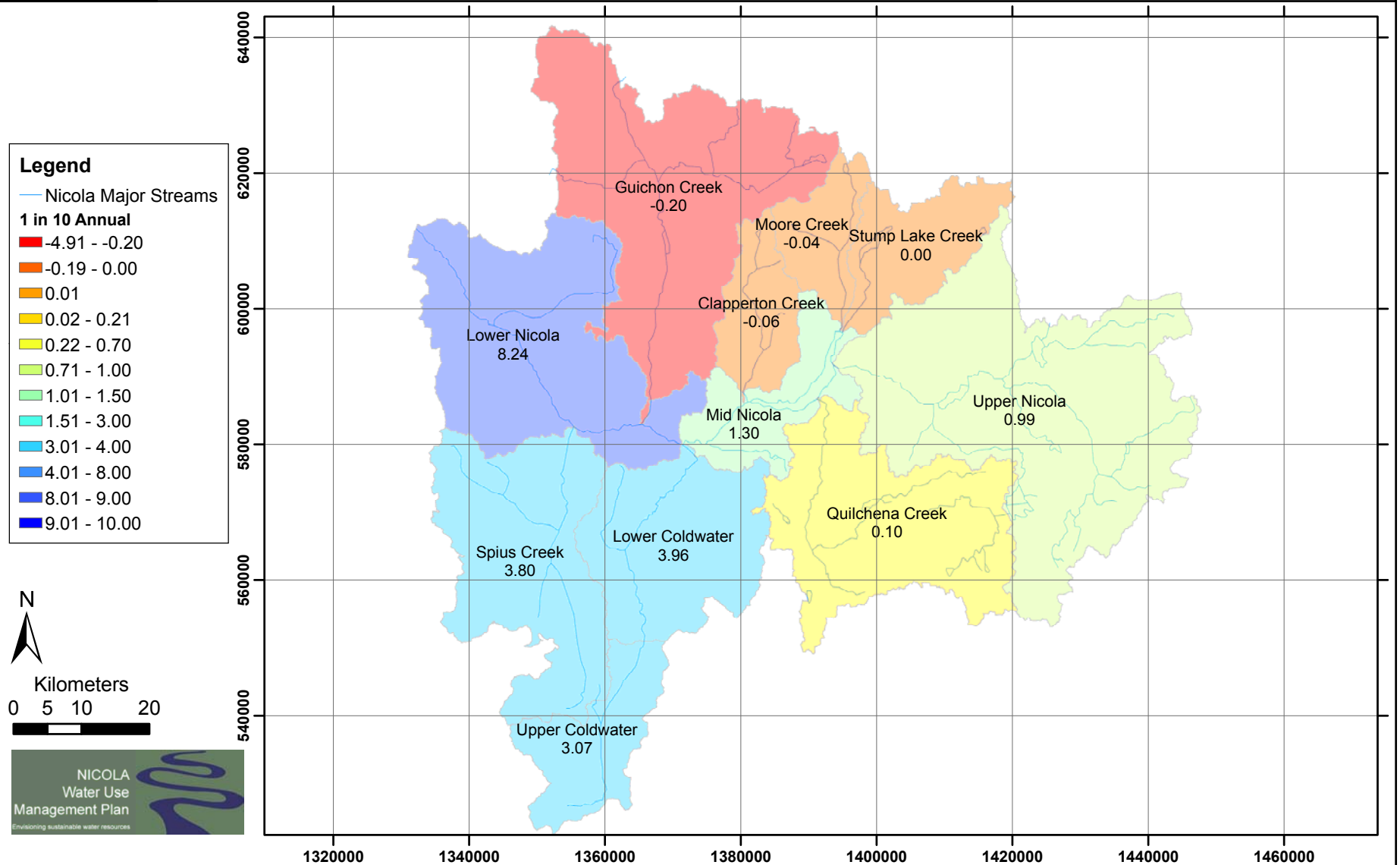
Figure 4 Current Conditions: Annual water budget in m 3 /s for 1 in 10 year drought
