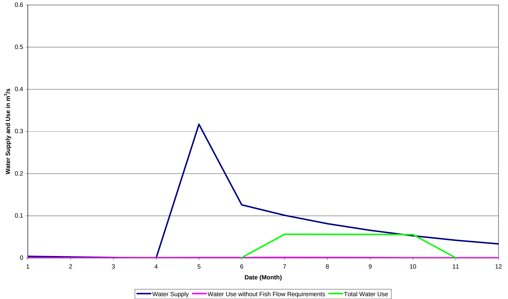
Figure 9: Water Supply and Use for Typical 1 in 10 year Drought Conditions Clapperton
