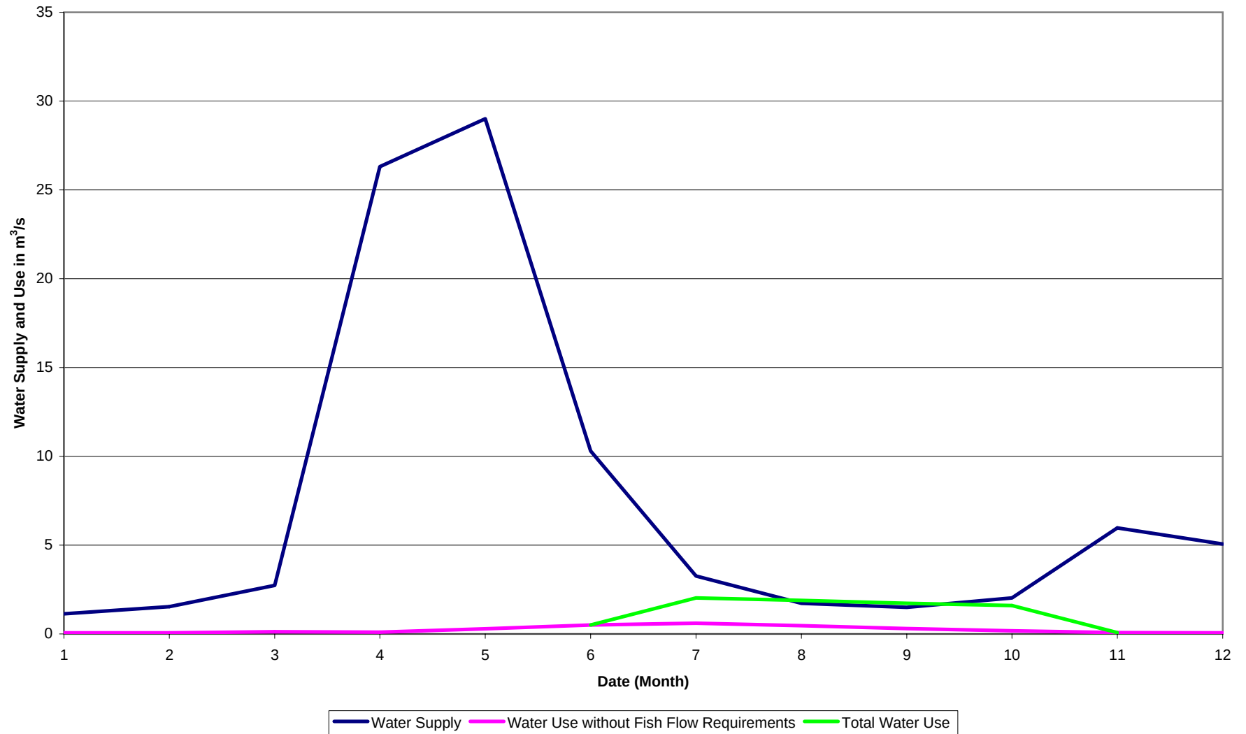
Figure 11: Water Supply and Use for Typical 1 in 10 year Drought Conditions Lower Coldwater
